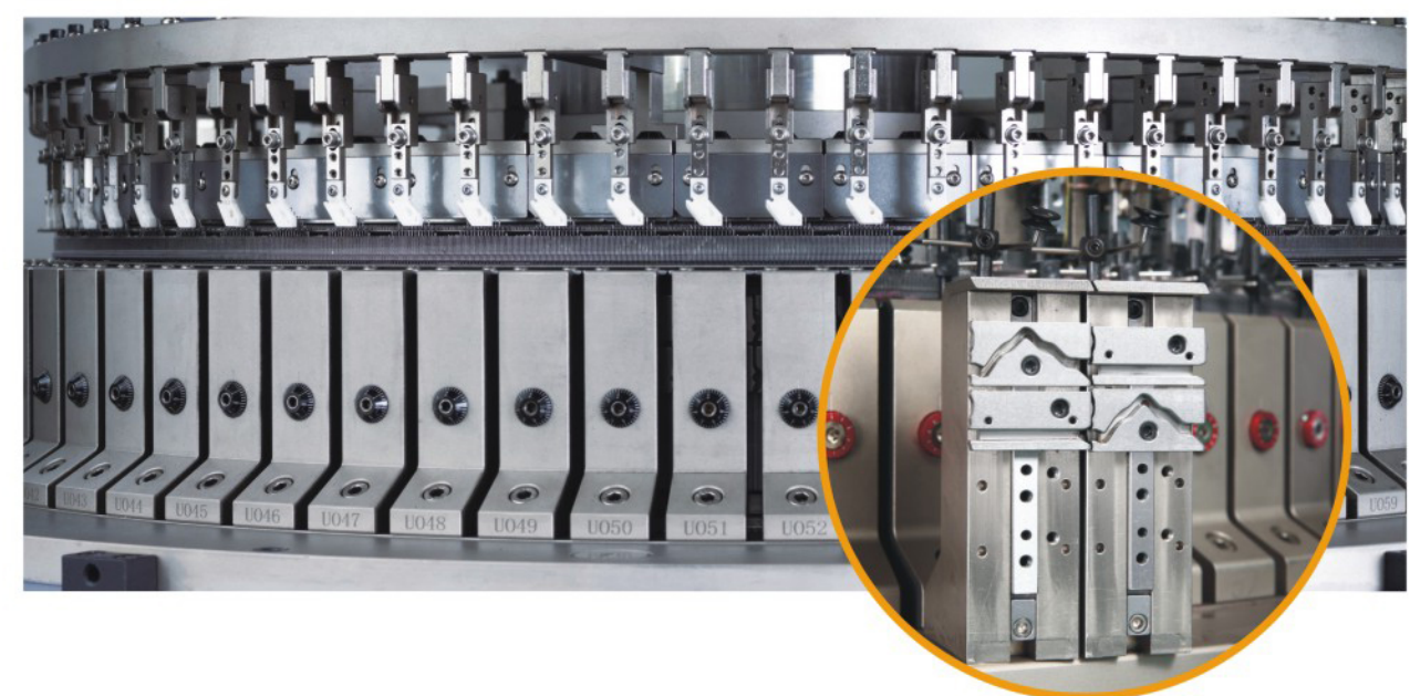
HX-L-KD 专用部件 THE PARTS FOR HX-L-KD ONLY
